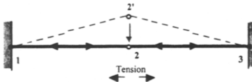
Figure 5.24 Tension pre-stress
