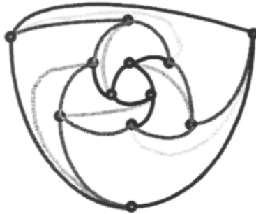
Figure 6.6 Complete cable-graph of a six-strut tensegrity module
