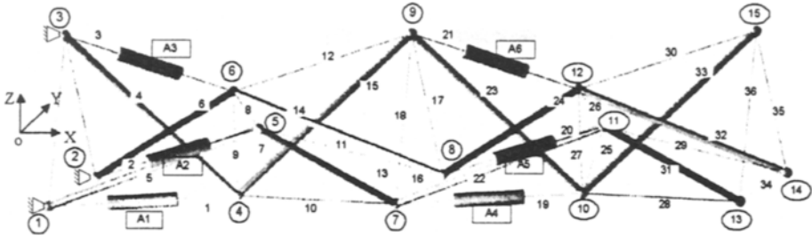
Figure 5.48 Tensegrity beam
