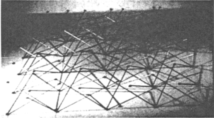
Figure 4.41 Double layer plane tensegrity grid
