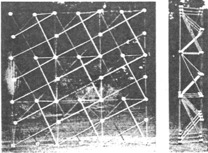
Figure 4.43 Double layer plane tensegrity grid (1992)
