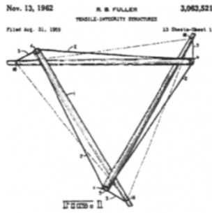
Figure 2.3 Fuller's patent
