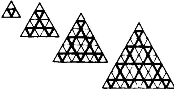
Figure 4.16 Distribution of struts and cables on a geodesic pattern
