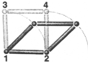
Figure 3.14 Finite mechanism
