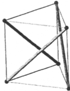
Figure 3.9 Cinematically indeterminate system (finite mechanism). First geometry
