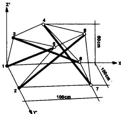
Figure 5.35 Quadruplex
