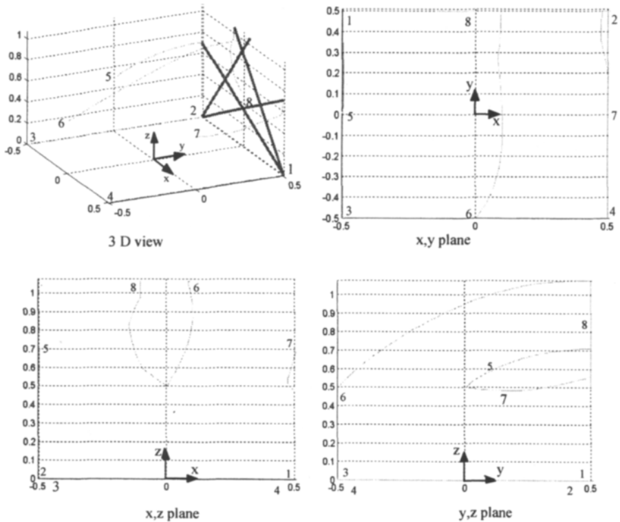
Figure 6.35 Node trajectories
