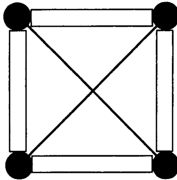
Figure 3.20 Equilibrium of bidimensional self-stress
