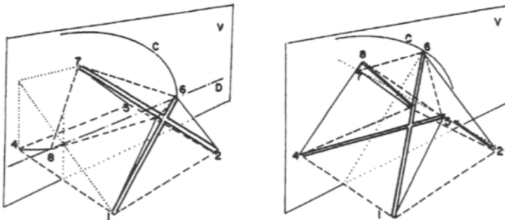
Figure 4.47 Strut-strut contacts limiting the trajectory
