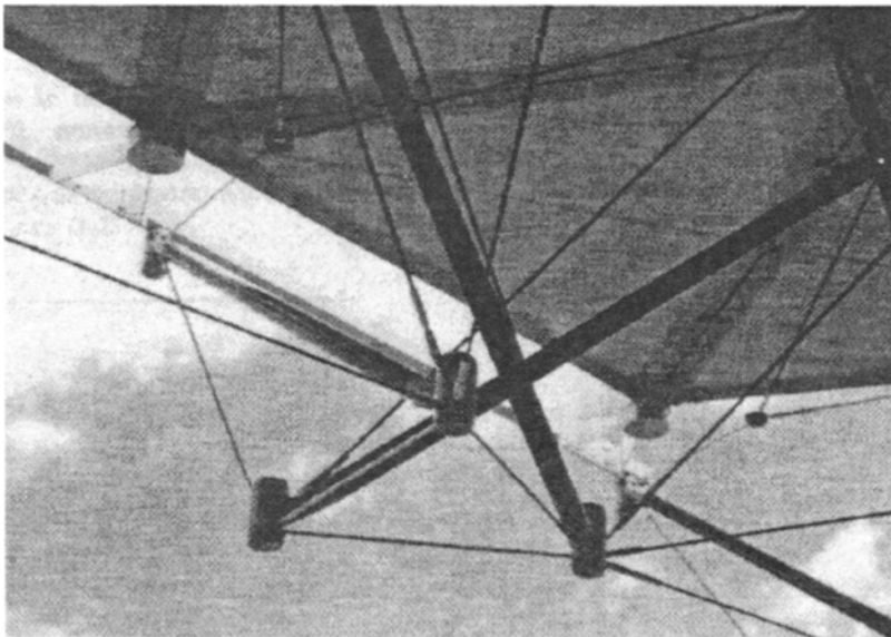
Figure 7.25 Kono's project
