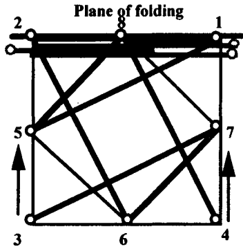
Figure 6.11 Mechanism activation
