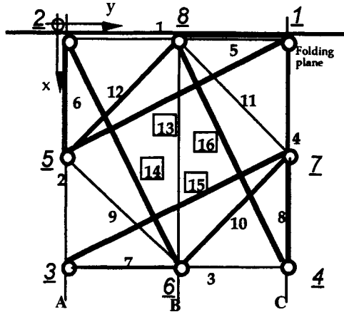
Figure 6.31 Numbering of nodes (italic, underlined) and members
