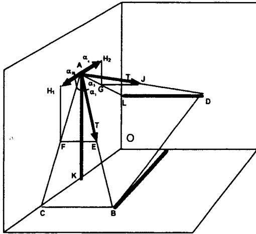
Figure 5.17 Expanded octahedron. Node equilibrium and form-finding
