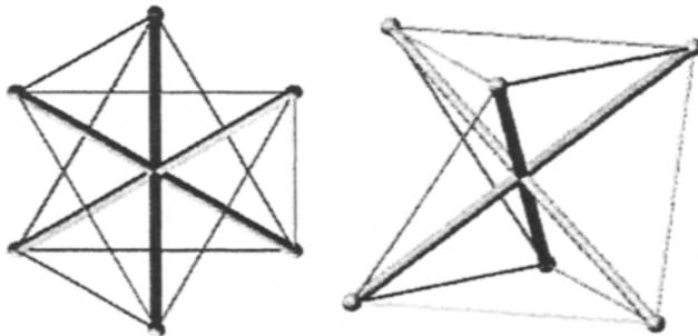
Figure 3.10 Cinematically indeterminate system (finite mechanism). Second geometry
