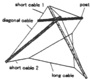
Figure 4.36 Elementary cell
