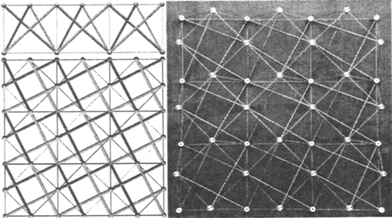
Figure 7.1 Double layer tensegrity grid (R. Motro, 1990)
