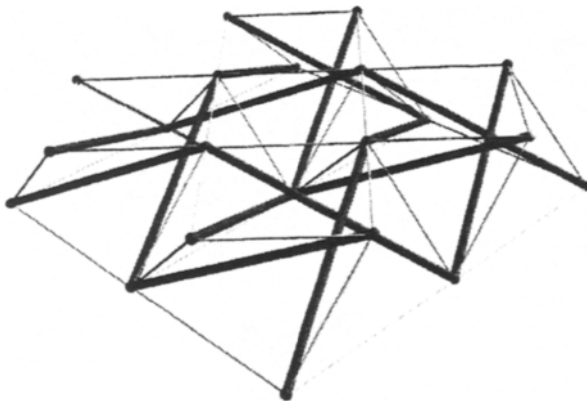
Figure 2.19 Complete grid
