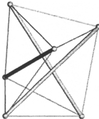
Figure 2.11 Self-stressed space structure. Elementary equilibrium
