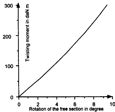
Figure 5.38 Torsion
