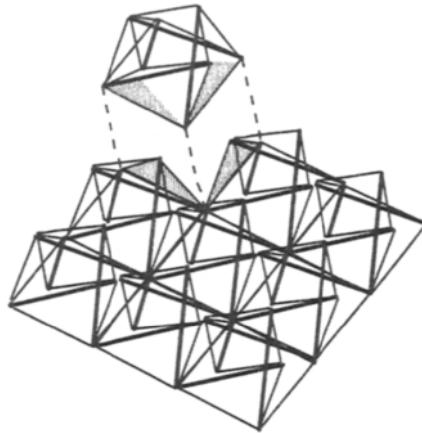
Figure 4.39 Double layer tensegrity grid principle: axonometric view
