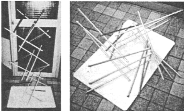
Figure 6.22 Physical model of a tensegrity mast
