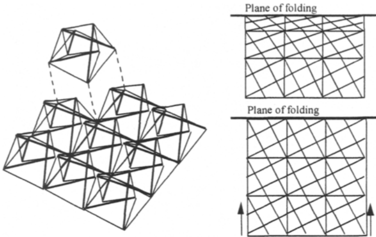
Figure 6.23 Tensegrity double layer grid folding policy
