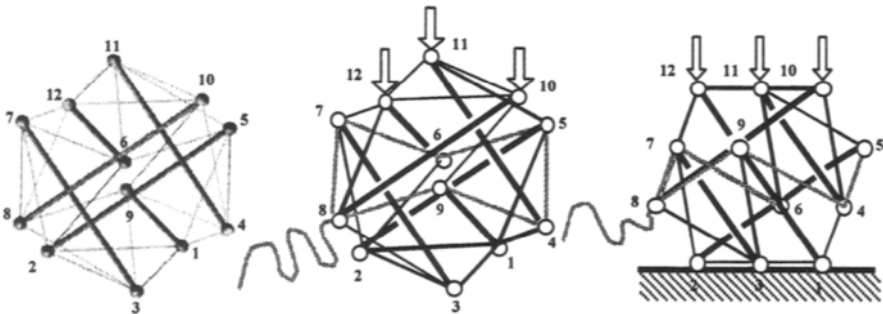
Figure 6.16 Folding with an active cable
