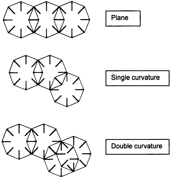
Figure 2.17 Structural situation diagrams
