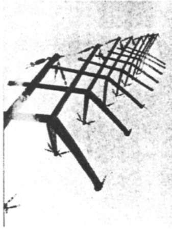
Figure 4.28 University of Oregon tensegrity mast, 1953
