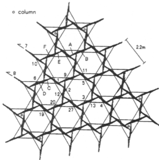
Figure 4.35 Plane double layer grid by Kono
