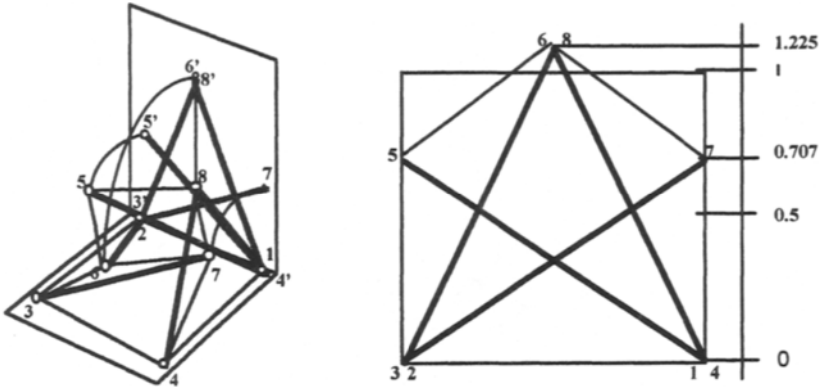
Figure 6.13 Nodes trajectories and final configuration
