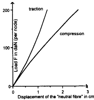
Figure 5.36 Compression and traction
