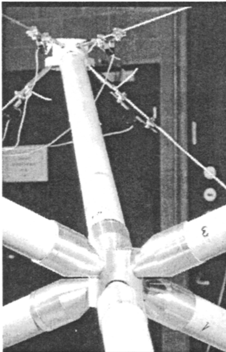
Figure 7.32 Central node
