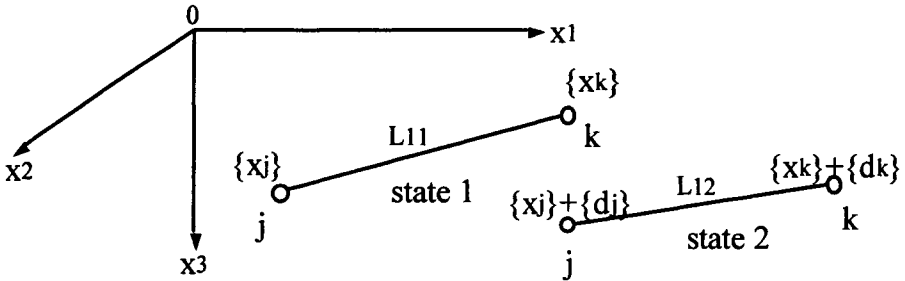
Figure 6.36 Displacement increments
