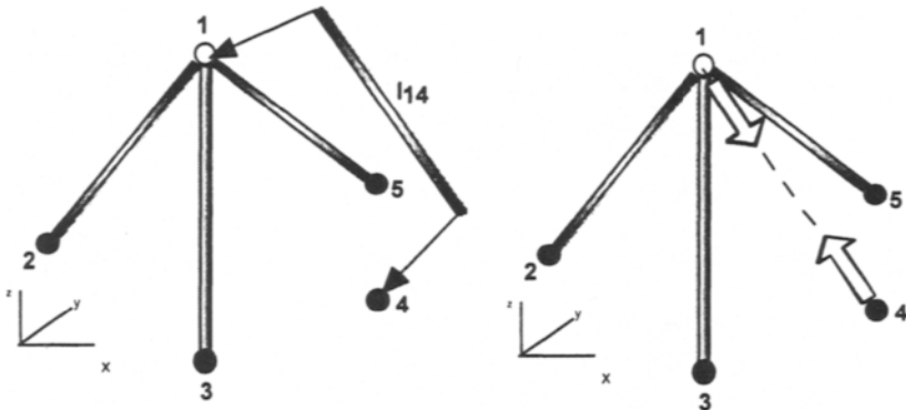
Figure 3.17 Initially stressed state
