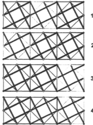
Figure 5.29 Feasible independent self-stress states
