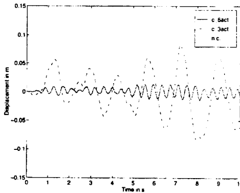
Figure 5.52 Variation with respect to Z-direction with 6, 3 or 0 actuators
