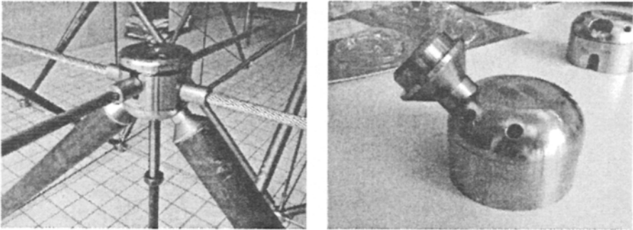
Figure 7.12 Assembly at node
