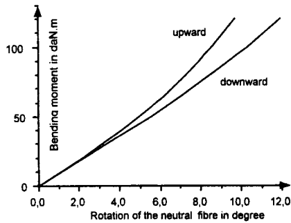
Figure 5.37 Flexion
